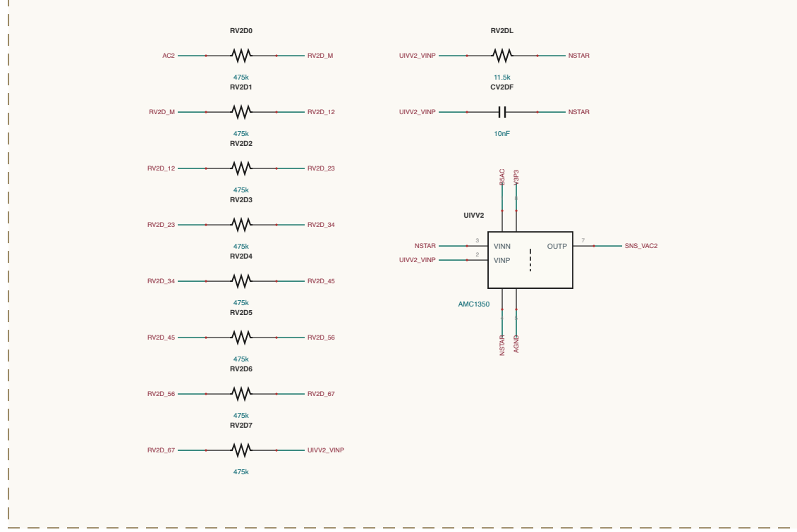
AC-SENSING / SENSE-VAC2
