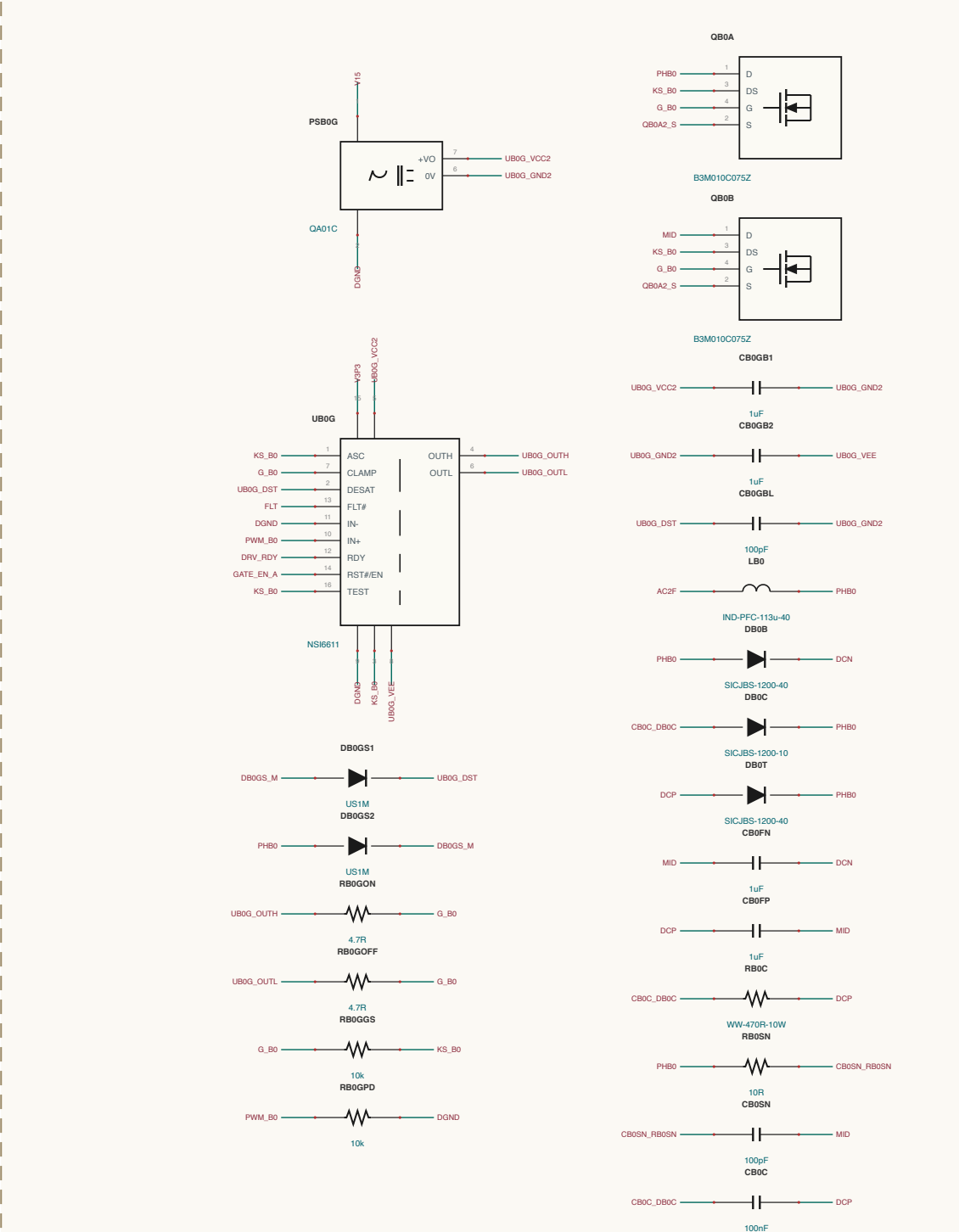
VIENNA-PFC / PHASE-B0
