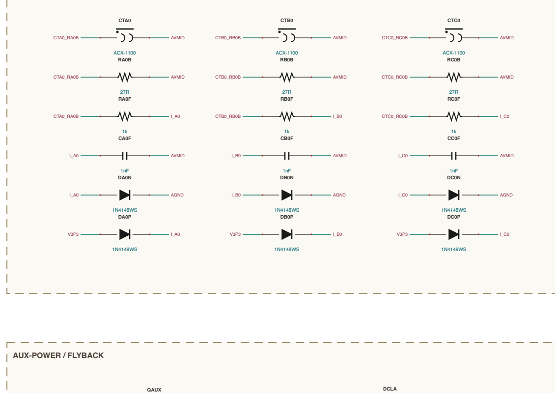
AC-SENSING / LINE-CTS-0
