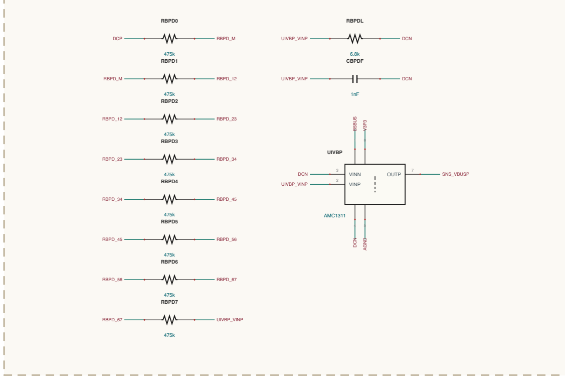
AC-SENSING / SENSE-VBUS
