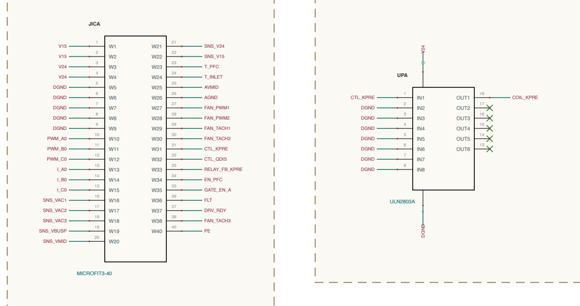
AUX-POWER / INTERCONNECT
