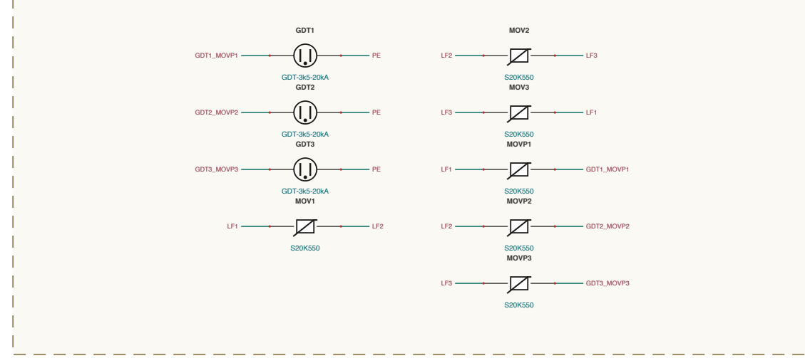
INPUT-EM / SURGE
