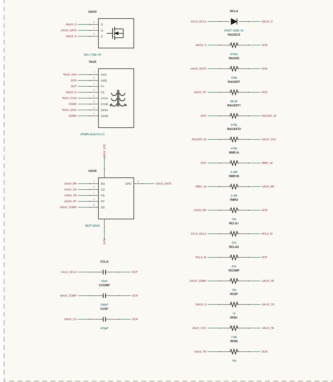
AUX-POWER / FLYBACK
