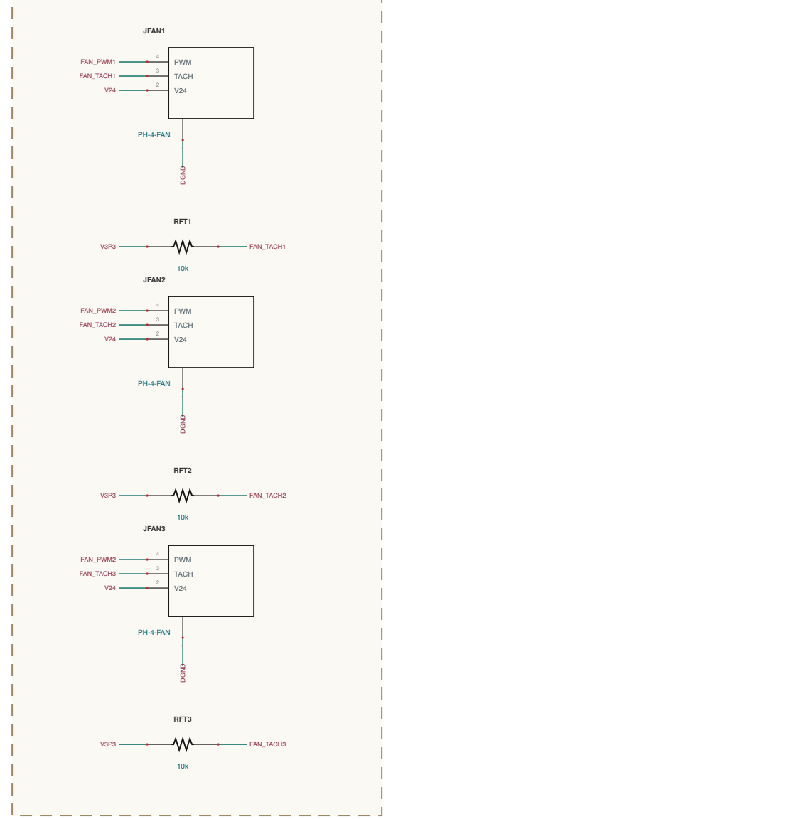
AUX-POWER / FANS
