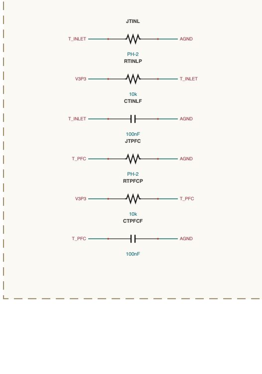
AC-SENSING / NTC
